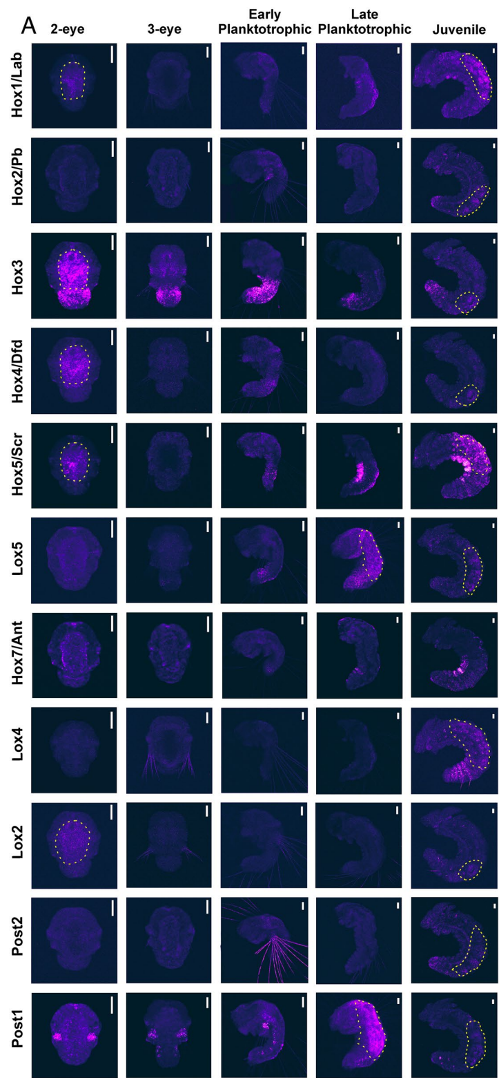
Fig. 4 A HCR in situ hybridization of the S. benedicti Hox genes at distinct developmental stages of the planktotrophic developmental mode. 2-eye and 3-eye stages are ventral view, and early planktotrophic, late planktotrophic, and juvenile are lateral view. Yellow dashed lines encircle confirmed autofluorescent regions. Scale bars = 50 \mu m. B HCR in situ hybridization of the S. benedicti Hox genes at distinct early developmental stages of the lecithotrophic developmental mode. 2-eye and 3-eye stages are ventral view, and early planktotrophic, late planktotrophic, and juvenile are lateral view. Yellow dashed lines encircle confirmed autofluorescent regions. Scale bars = 50 \mu m
